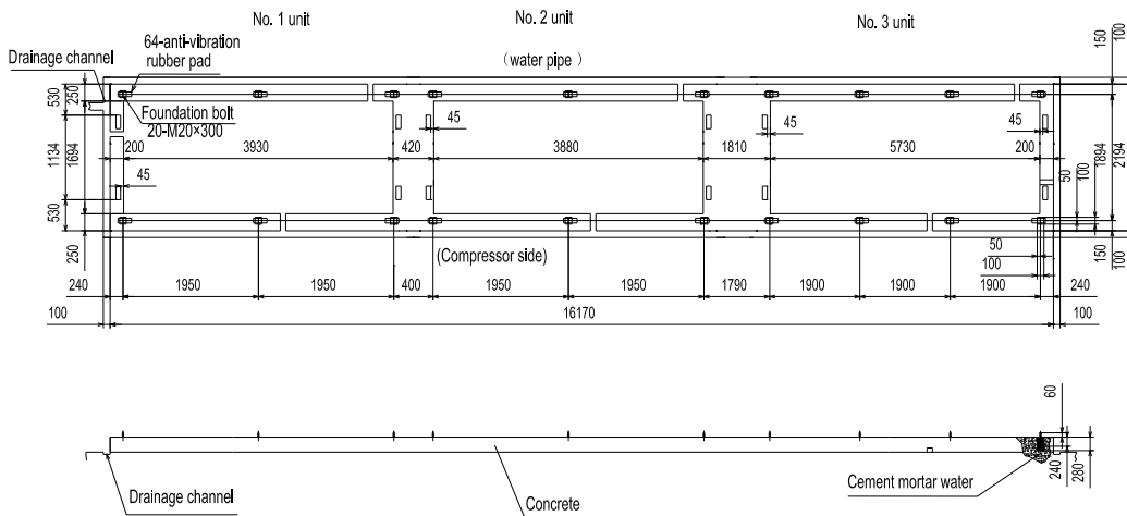
Detail drawing of foundation installation (not to scale)
