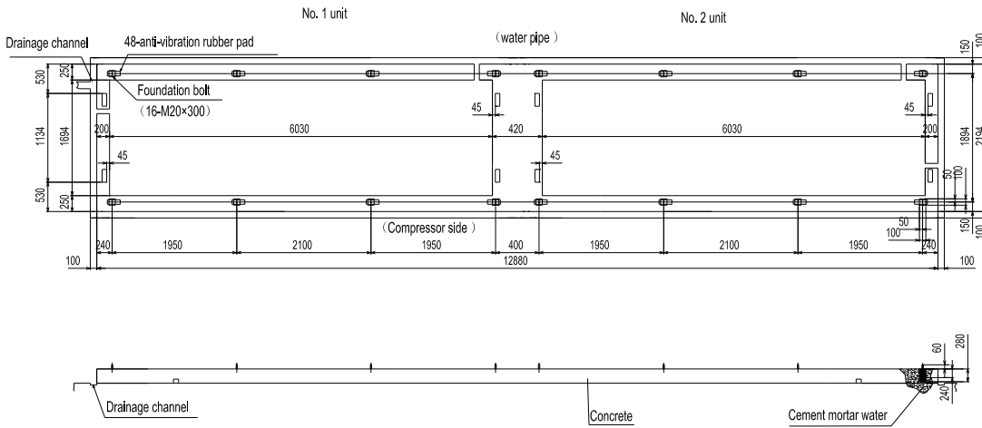
Detail drawing of foundation installation (not to scale)
