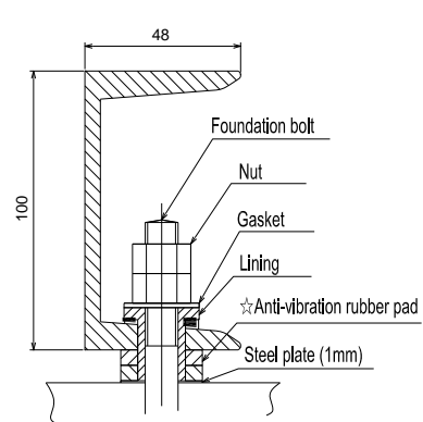
Detail drawing of foundation installation (not to scale)
