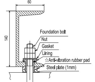
Detail drawing of foundation installation (not to scale)
