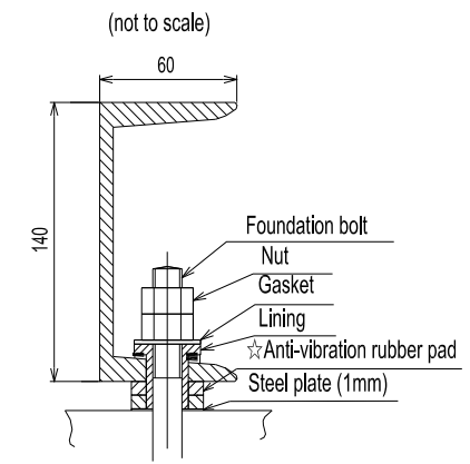
Detail drawing of foundation installation
